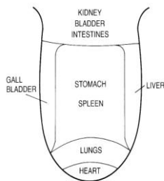
Fig. 54 Correspondence of tongue areas to organs
